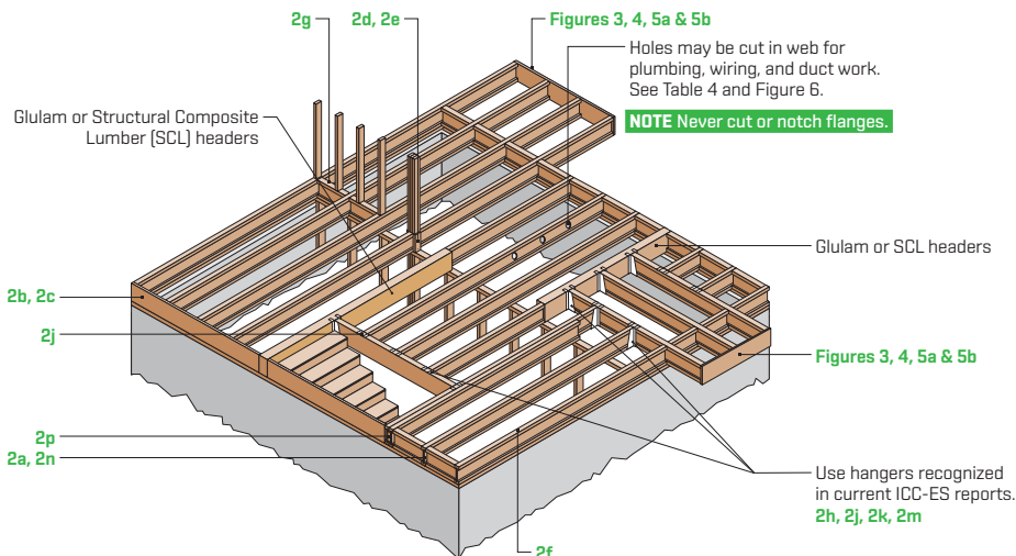
FIGURE 2 Typical P3 Floor Joist Framing and Construction Details
